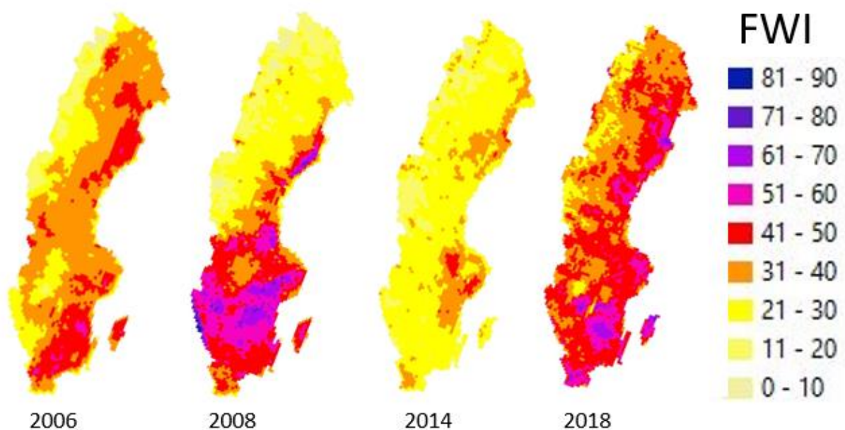
Figure 101. Example of years with major fires and the maximum value of the fire weather index (FWI). Note that the year 2014, when the major fire occurred in Västmanland (14 000 ha) only some smaller areas were affected by high danger.
