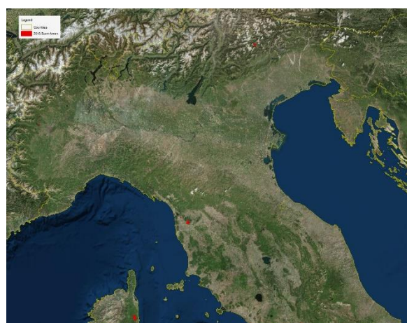
Figure 181. Burnt area scars in Pisa region in Italy.
