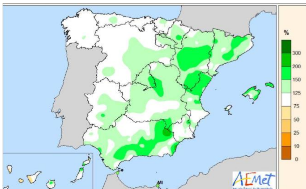
Figure 95. Percentage of accumulated precipitation in 2018 over the average (SOURCE: Meteorology Statat Agency. Ministry for the Ecological Transition).
