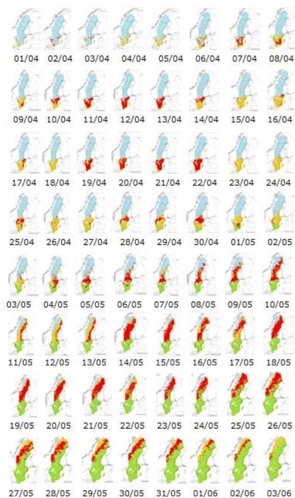
Figure 98. Maps of grass fire risk season 2018 shows periods of risk in combination with snow.
