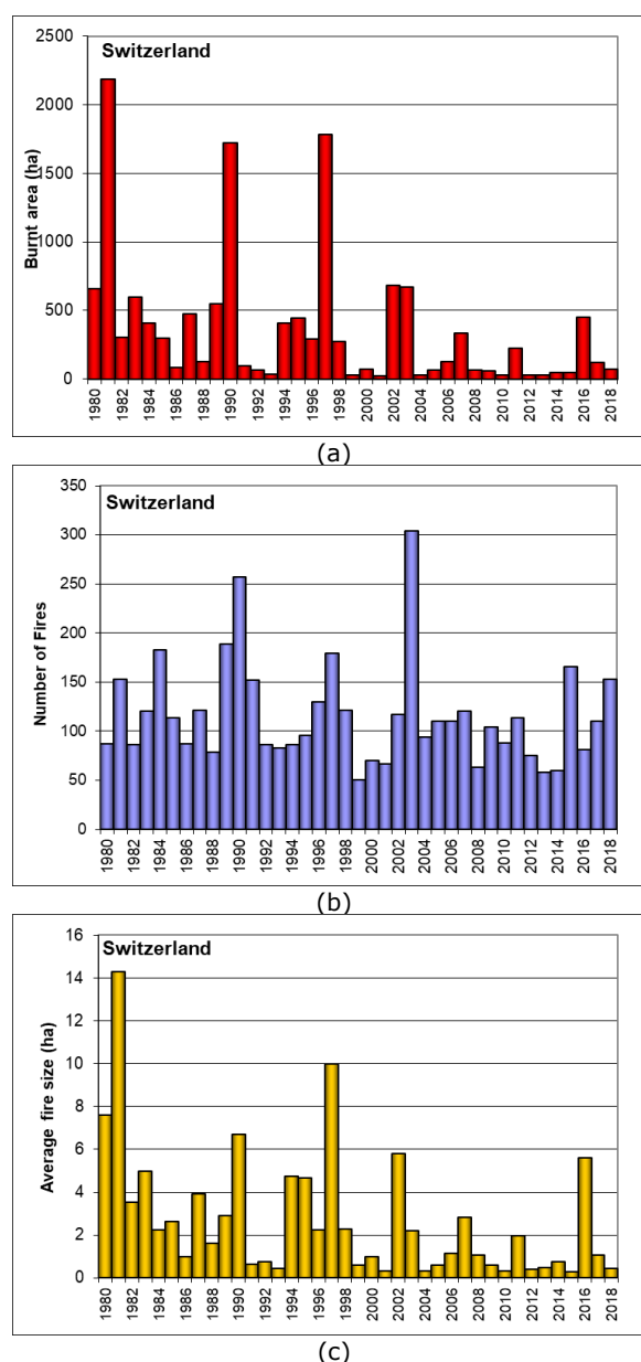
Figure 107. Burnt areas (a), number of fires (b) and average fire size (c) in Switzerland from 1980-2018.
