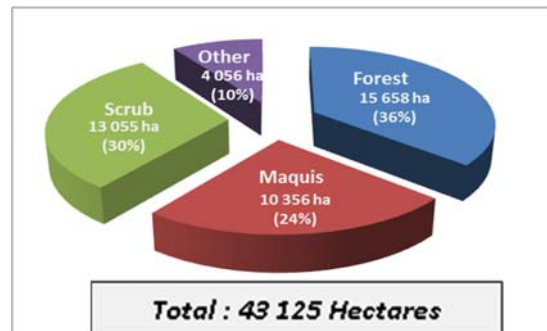
Figure 85. Burnt area classified by vegetation type
