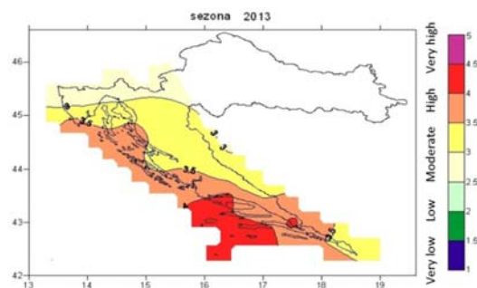
Figure 5. Average monthly Fire Danger Rating for forest fires for June 2013.
